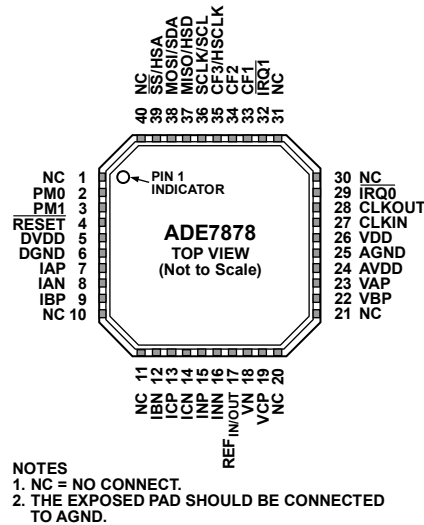
Figure 6. Pin Configuration
