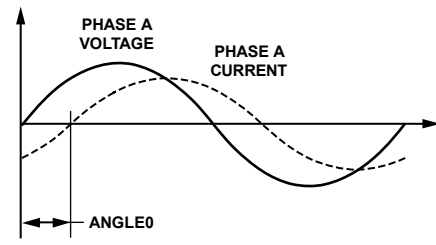
Figure 44. Delay Between Phase A Voltage and Phase A Current Is Stored in ANGLE0[15:0]
