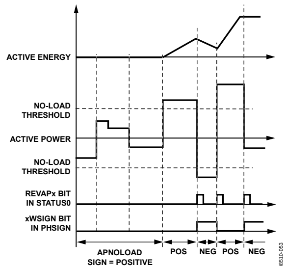
Figure 72. Active Power Signed Accumulation Mode
