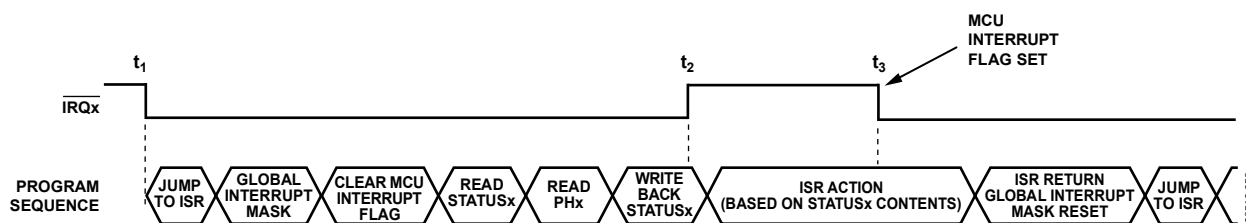
Figure 79. Interrupt Management When PHSTATUS, IPEAK, VPEAK, or PHSIGN Registers Is Involved
