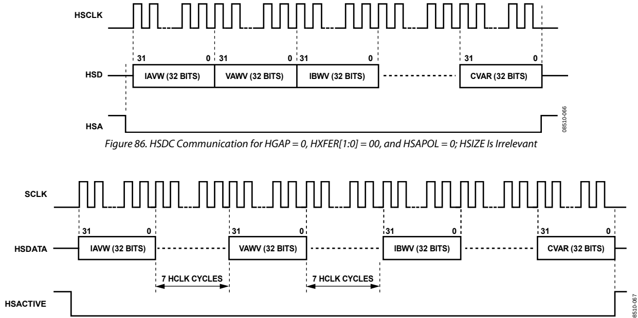
Figure 87. HSDC Communication for HSIZE = 0, HGAP = 1, HXFER[1:0] = 00, and HSAPOL = 0
