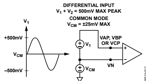
Figure 26. Maximum Input Level, Voltage Channels, Gain = 1
