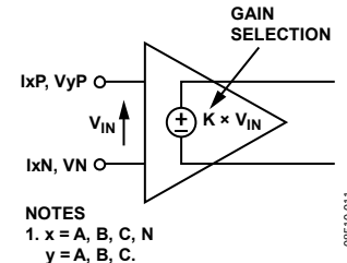
Figure 25. PGA in Current and Voltage Channels
