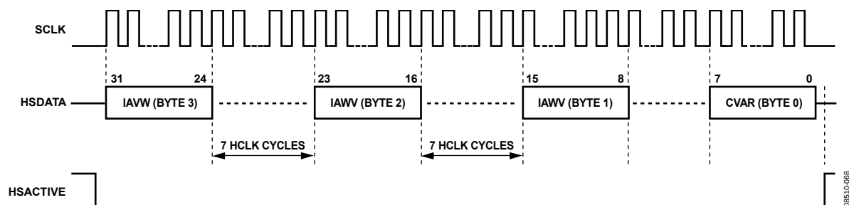
Figure 88. HSDC Communication for HSIZE = 1, HGAP = 1, HXFER[1:0] = 00, and HSAPOL = 0
