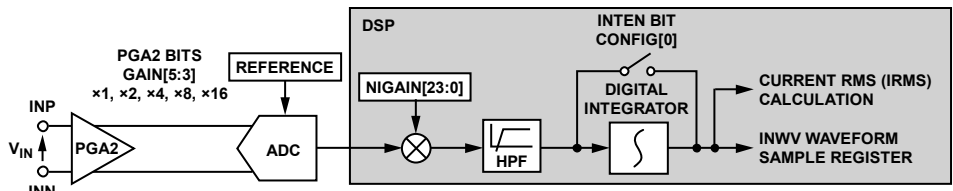
Figure 31. Neutral Current Signal Path
