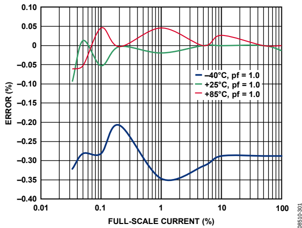
Figure 7. Total Active Energy Error As Percentage of Reading (Gain = +1, pf = 1 ) over Temperature with Internal Reference and Integrator Off
