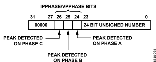
Figure 47. Composition of IPEAK[31:0] and VPEAK[31:0] Registers
