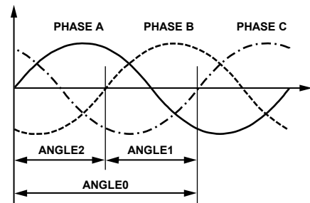
Figure 45. Delays Between Phase Voltages (Currents)
