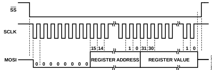
Figure 84. SPI Write Operation of a 32-Bit Register
